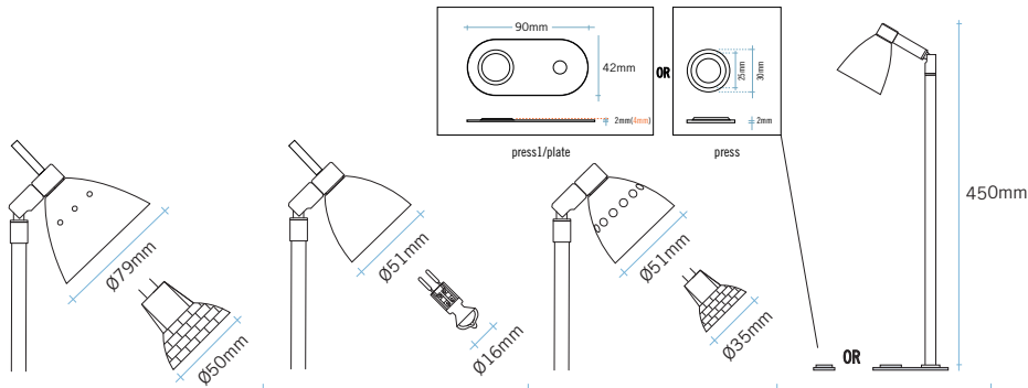
AL-07/Y Ø50mm dichroic or reflector halogen lamp: 20W 35W 50W
